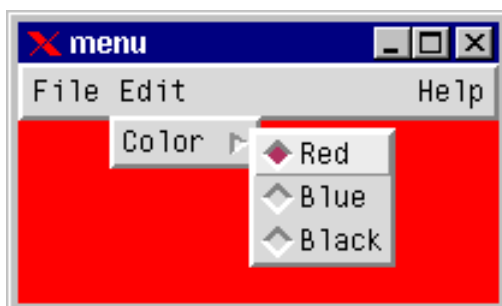
Figure 1.22: Simple Menu
