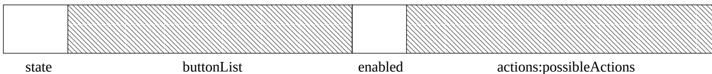
Figure 1.1: Figure symbolizes the bytes of a Window:status message. The components buttonList and actions are excluded from decode. Only state and enabled are decoded when decode__Window_exclusive is called.
