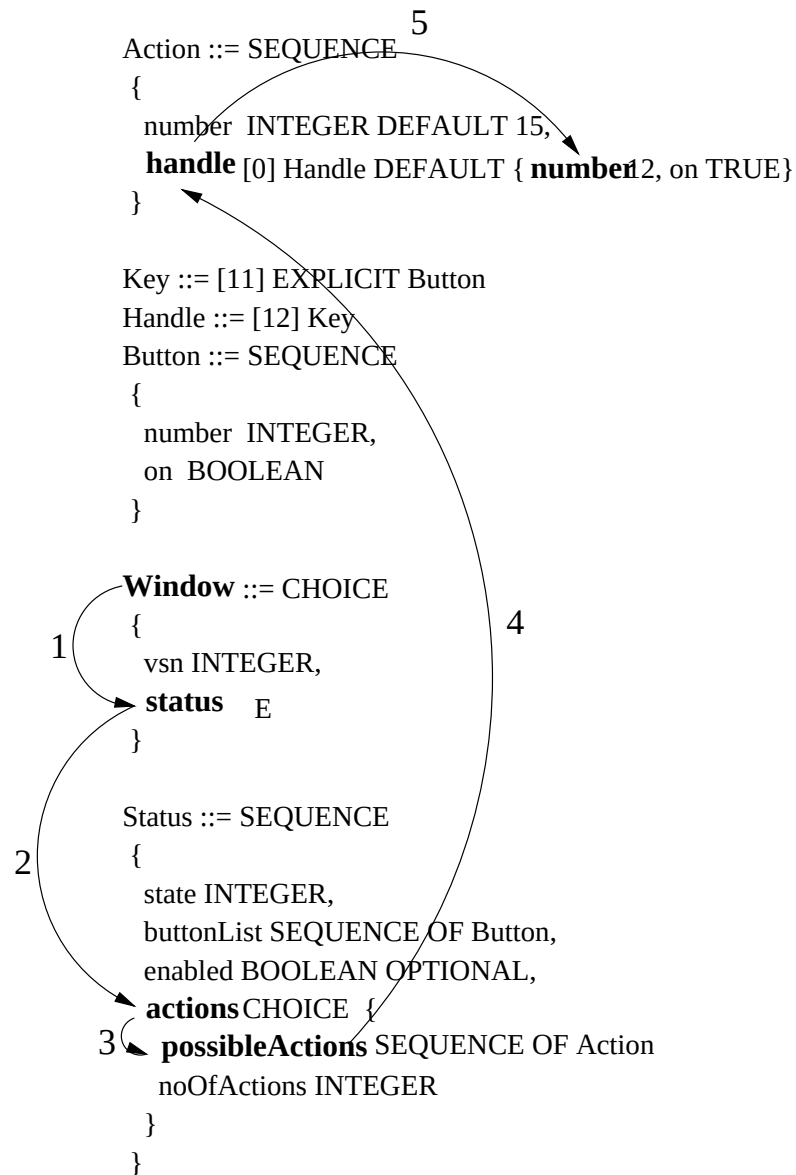
Figure 1.2: The elements specified in the config file for selective decode of a sub-value in a Window message
