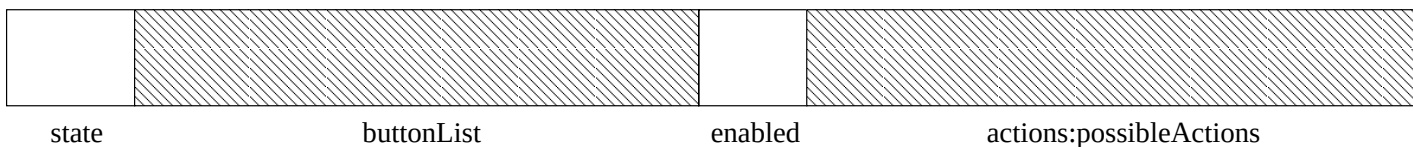
Figure 1.1: Figure symbolizes the bytes of a Window:status message. The components buttonList and actions are excluded from decode. Only state and enabled are decoded when decode_Window_exclusive is called.
