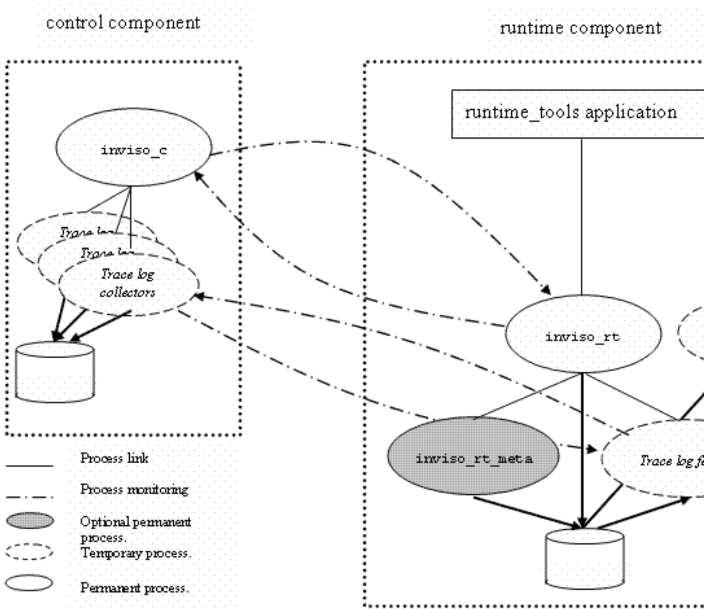
Figure 1.1: Inviso Trace System Architecture Overview.
