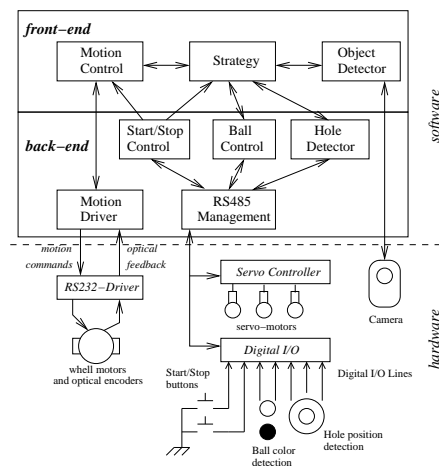
Fig. 3. Hardware/Software Architecture
