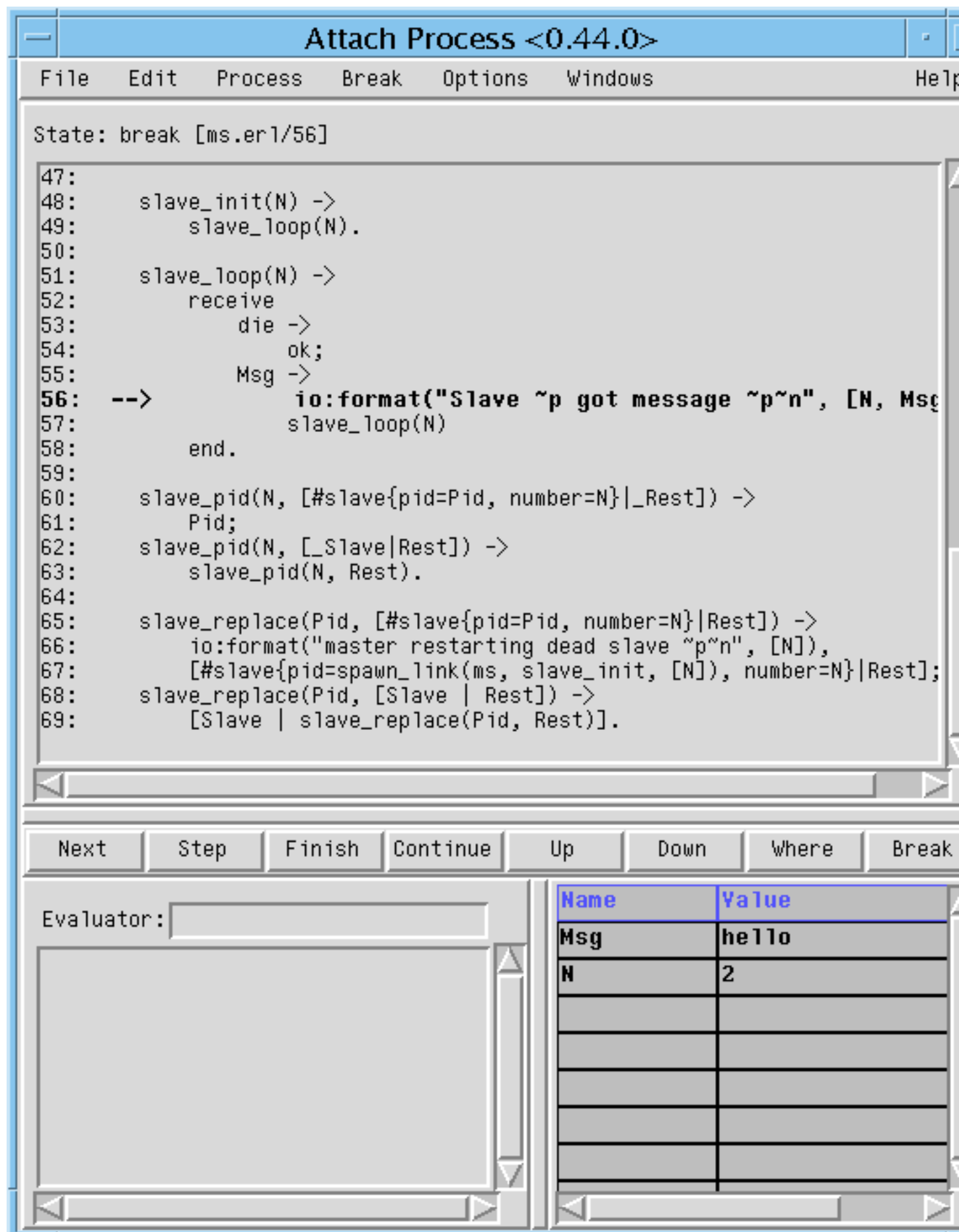
Figure 1-6 The Attach Process (DBL) Debugger
