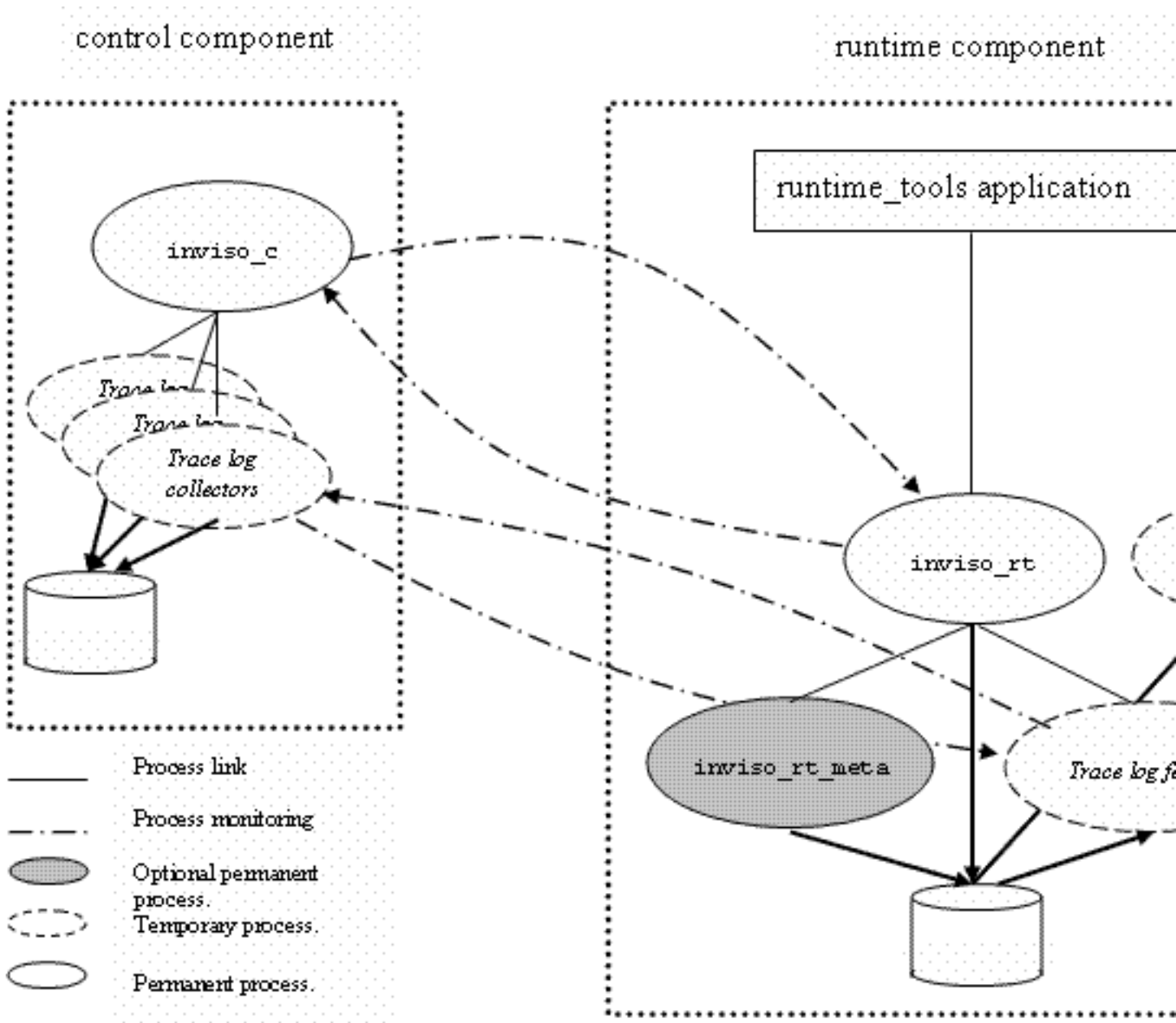
Figure 1.1: Inviso Trace System Architecture Overview.
