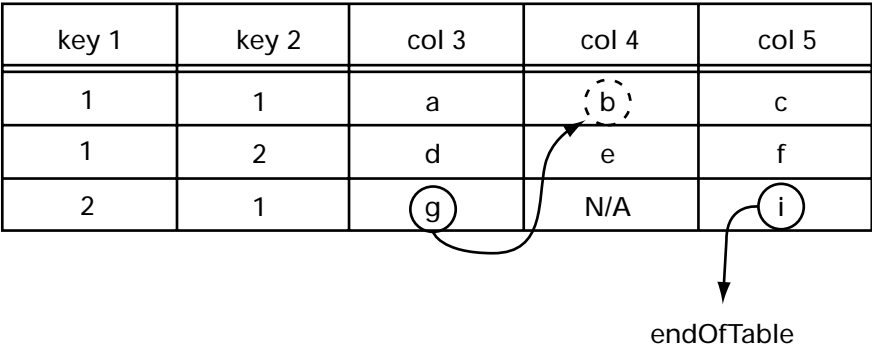
Figure 1.7: GetNext from [3,2,1] and [5,2,1].
